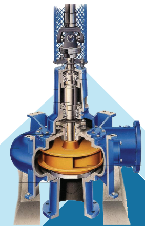
Large dry pit
